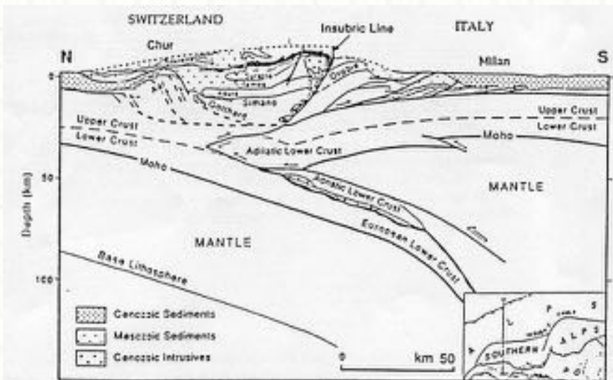
Fig. 39 - Interpretative cross section of the Alps between Switzerland and Italy, after Pfiffner, in Blundell et al. (1992).
